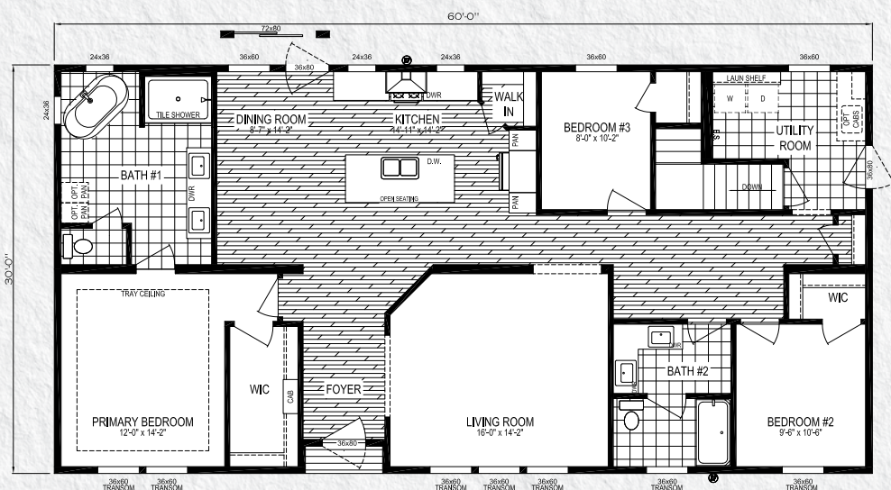
Basement Layout
